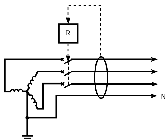
Fig. 16: Zero sequence.
